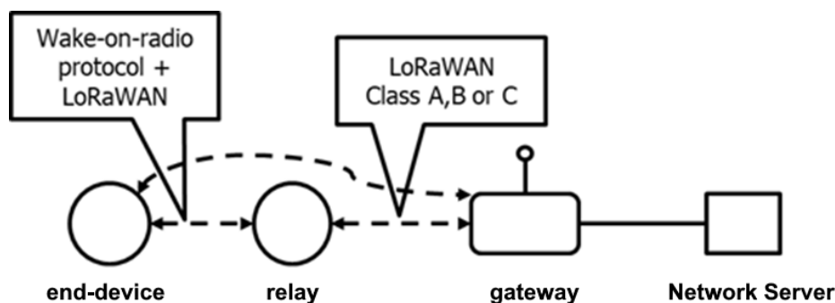
Figure 2 LoRaWAN Relay mechanism principle
