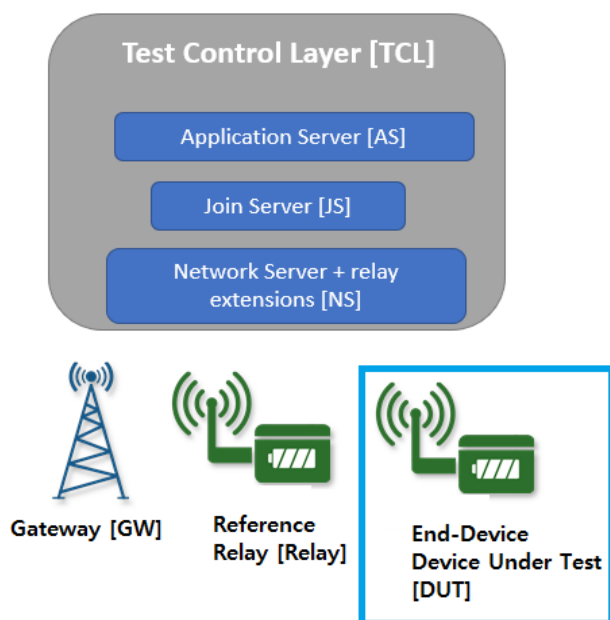
Figure 1 Test Harness Architecture when the DUT = End-Device
